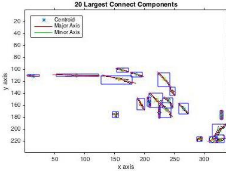
Figure 4. Geometric properties of the 20 largest connected component of the stress crack.
