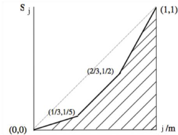
Figure 2. An example of Lorentz information curve of L = 3 .
